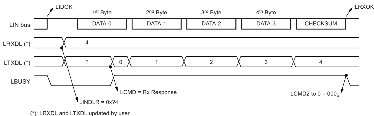
Figure 5-76. LIN 2.1 - Rx Response - No Error
