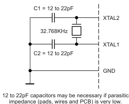
Figure 5-12. Low-frequency Crystal Oscillator Connections
