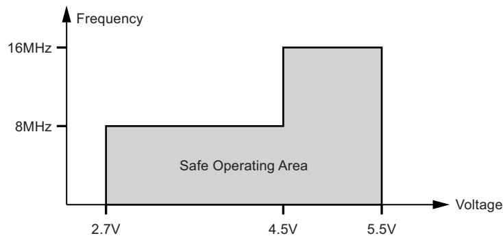
Figure 5-107. Maximum Frequency versus Vcc, Atmel® ATtiny87/167
