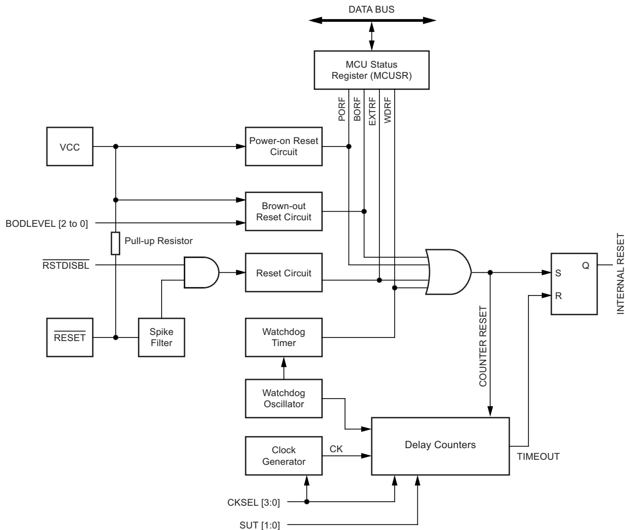
Figure 5-16. Reset Circuit
