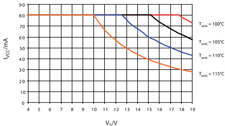
Figure 4-20. Power Dissipation: Safe Operating Area (SOA) of VCC Output Current vs Supply Voltage VS at Different Ambient Temperatures, and No Current Source (Pins CSx) Active
