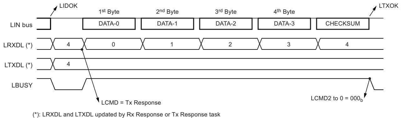
Figure 5-77. LIN 1.3 - Tx Response - No Error
