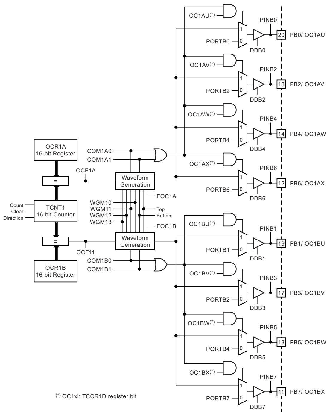
Figure 5-48. Compare Match Output
