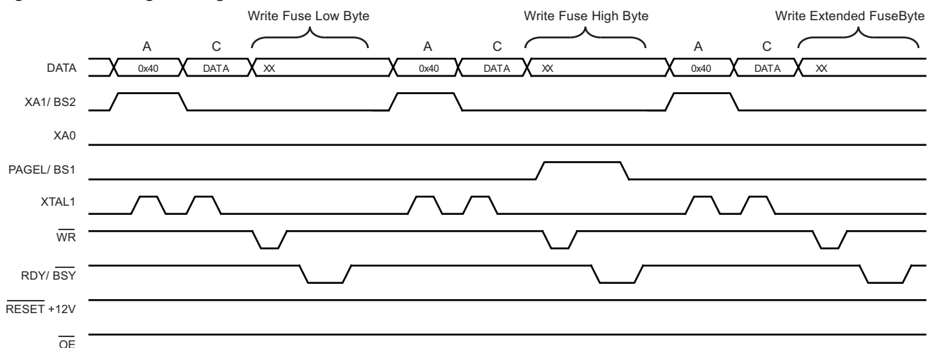
Figure 5-102. Programming the FUSES Waveforms
