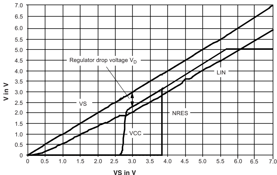
Figure 4-11. VCC versus VS
