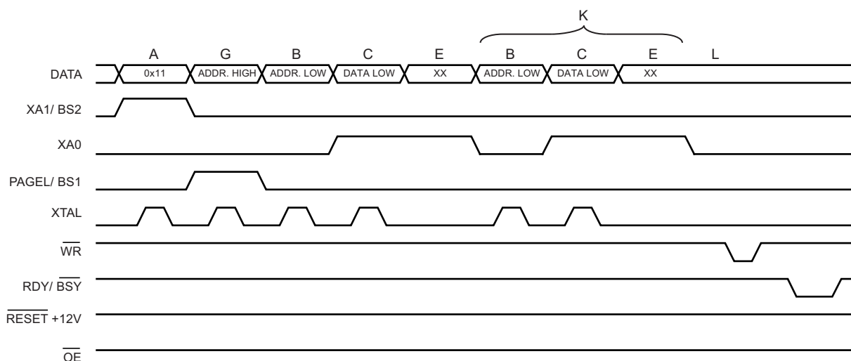
Figure 5-101. Programming the EEPROM Waveforms
