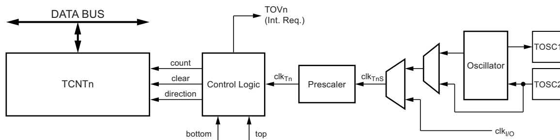
Figure 5-31. Counter Unit Block Diagram
