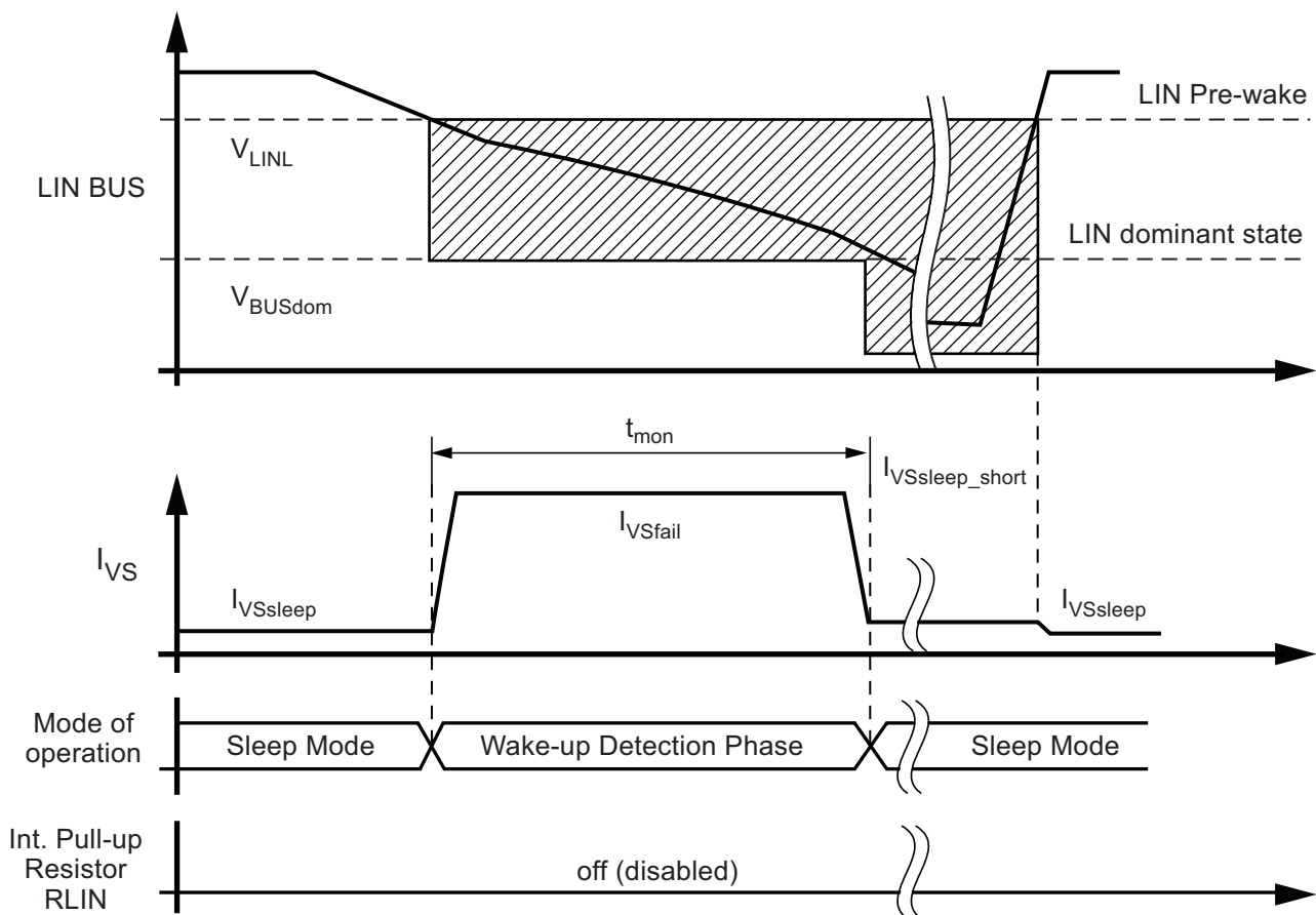
Figure 4-7. Floating LIN Bus During Sleep Mode
