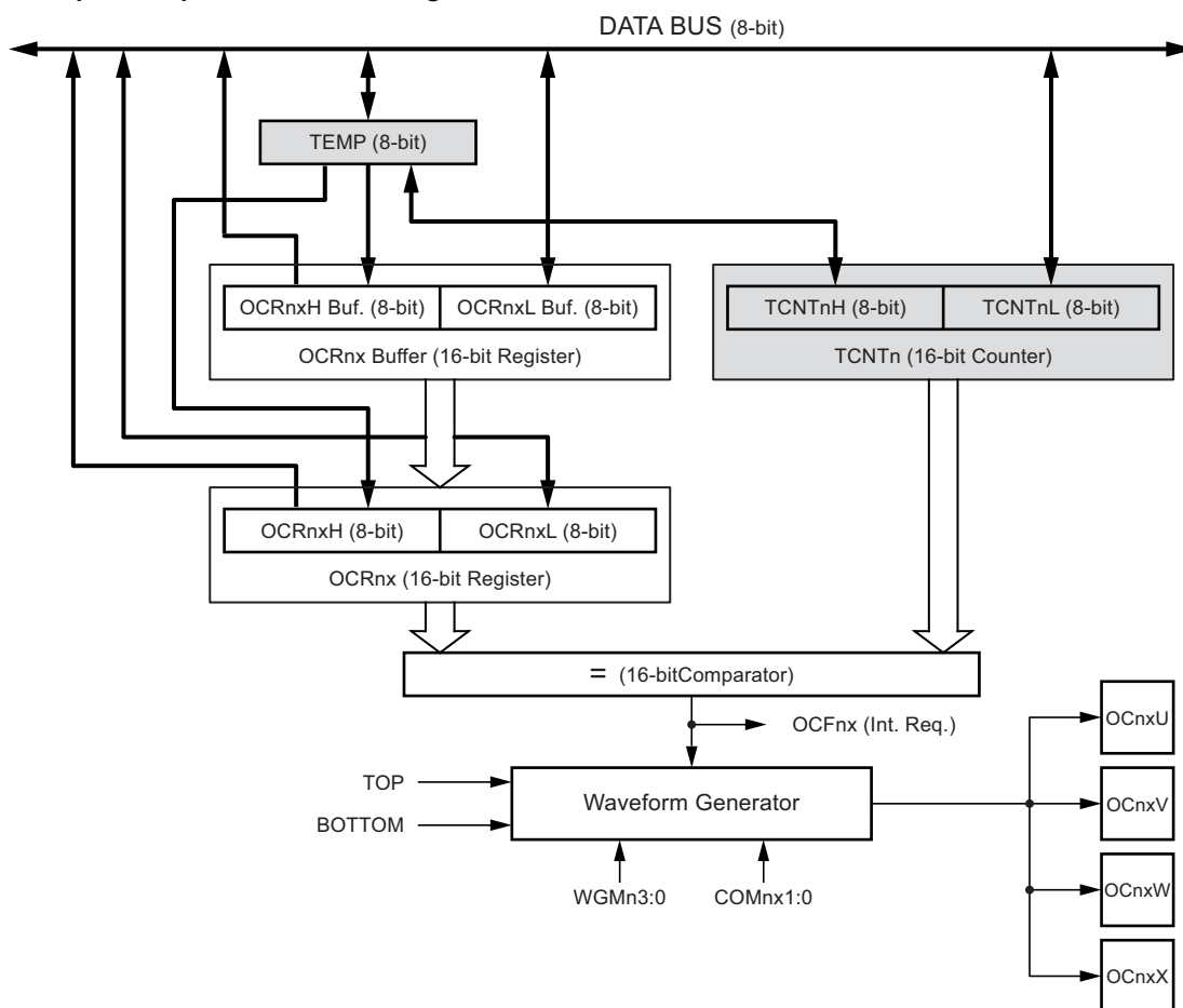
Figure 5-47. Output Compare Unit, Block Diagram
