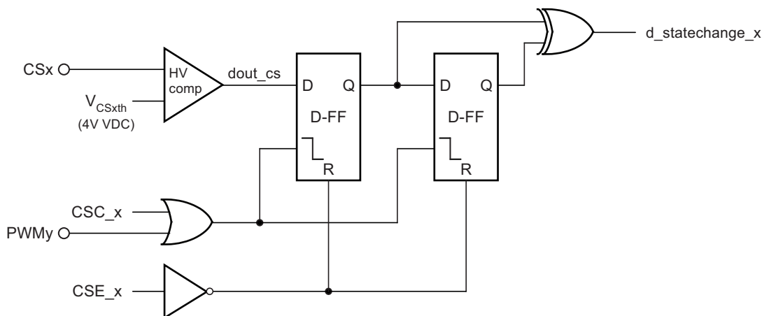
Figure 4-17. State Change Detection Circuitry
