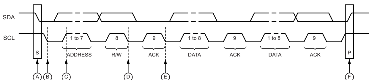
Figure 5-66. Two-wire Mode, Typical Timing Diagram
