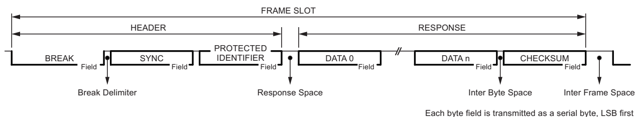
Figure 5-70. Structure of a LIN Frame
