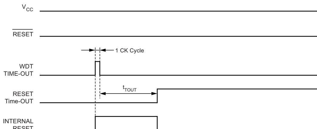
Figure 5-21. Watchdog System Reset During Operation
