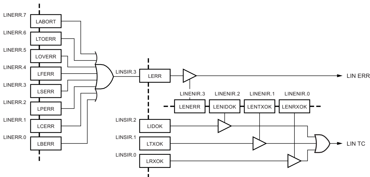
Figure 5-80. LIN Interrupt Mapping
