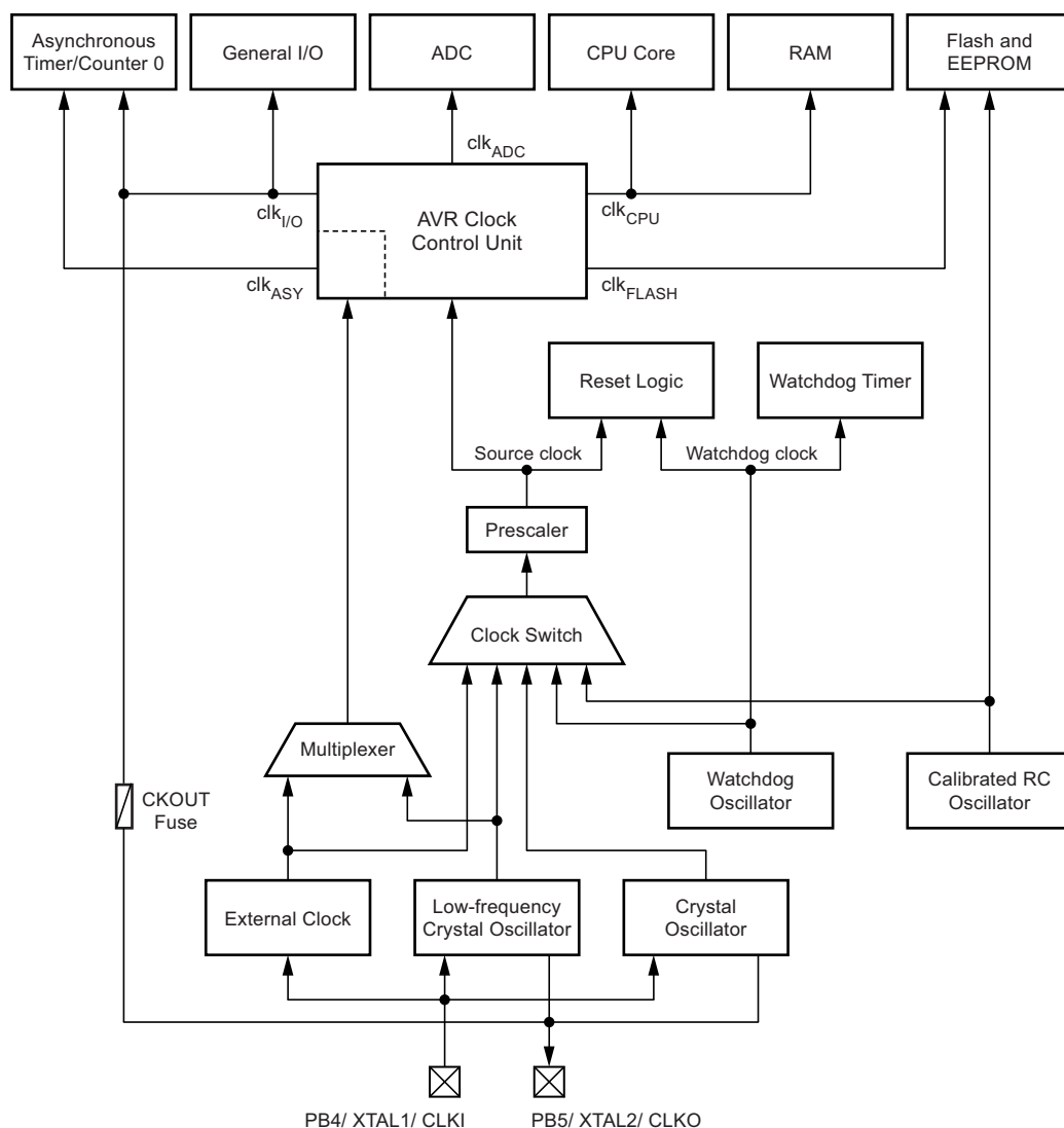
Figure 5-10. Clock Distribution
