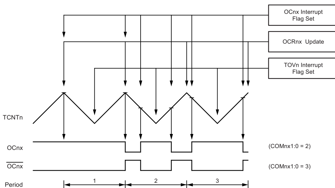
Figure 5-36. Phase Correct PWM Mode, Timing Diagram
